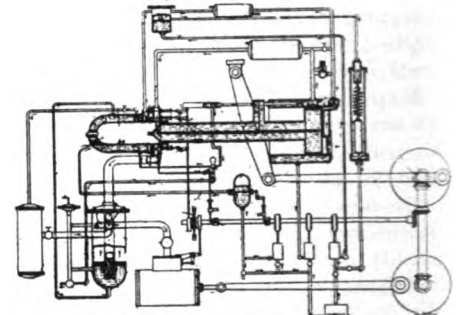
Reeve Compound Explosive Engine
